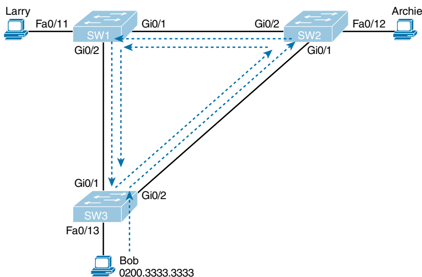
Figure 8-1 Broadcast Storm
