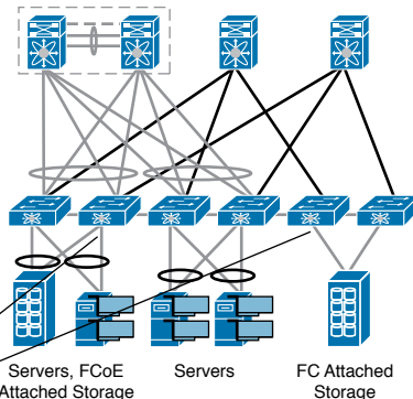
Figure 23-58 Unified Port Support on Nexus 5500 Series Switches
