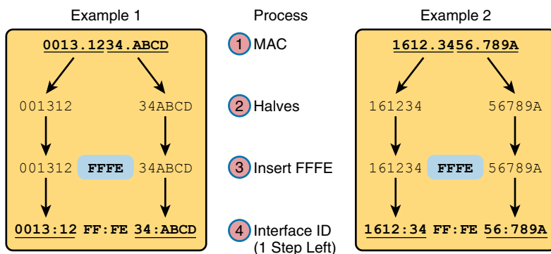
Figure 15-15 Two Examples of Most of the EUI-64 Interface ID Process
