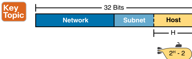
Figure 11-10 Subnet Size Concepts
