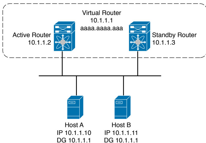
Figure 20-1 Communication Between Two Hosts in the Same Subnet
