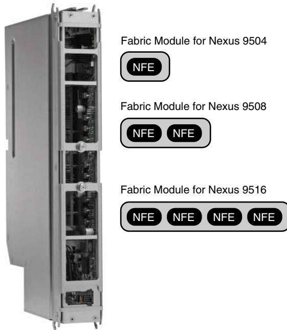
Figure 1-12 Nexus 9500 Fabric Module
