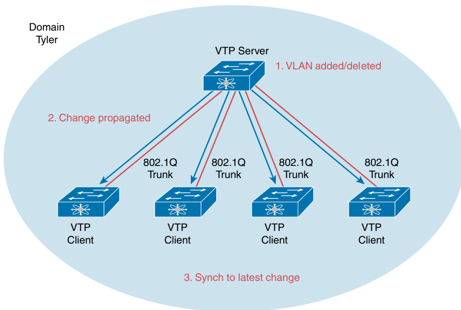
Figure 7-3 VTP Operation
