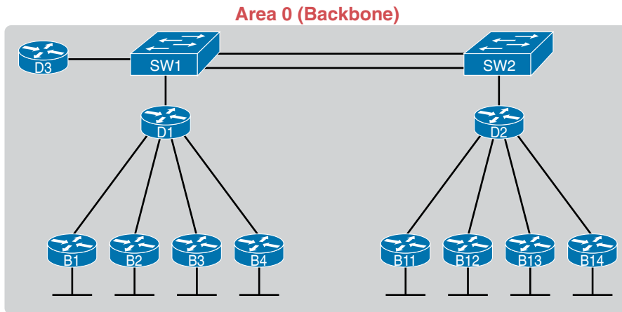
Figure 18-15 Single-Area OSPF
