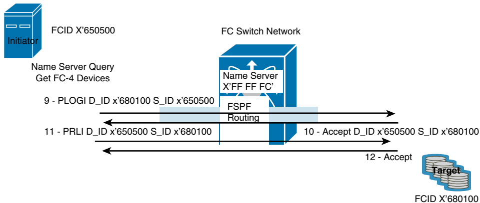
Figure 22-30 Fibre Channel Port/Process Login to Target
