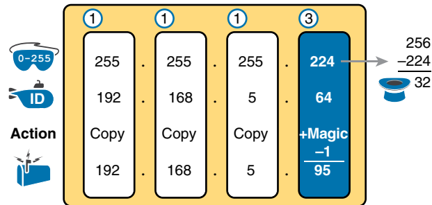
Figure 14-12 Find the Subnet Broadcast: 192.168.5.64, 255.255.255.224
