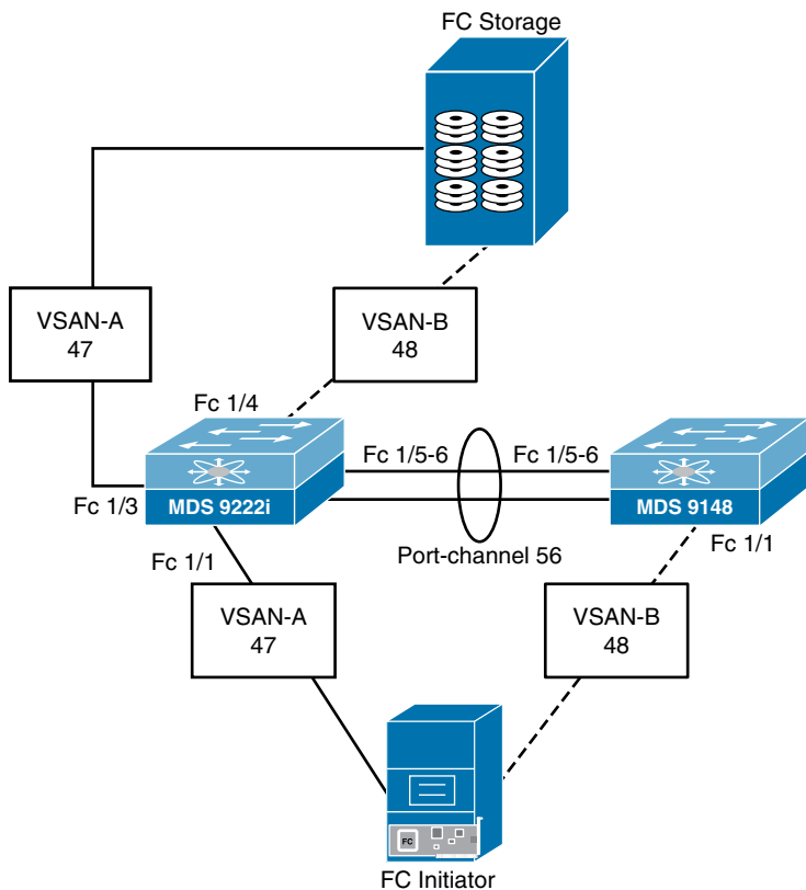
Figure 23-33 Our Sample SAN Topology Diagram
