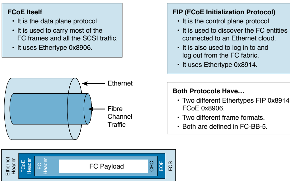
Figure 23-48 FCoE Protocols
