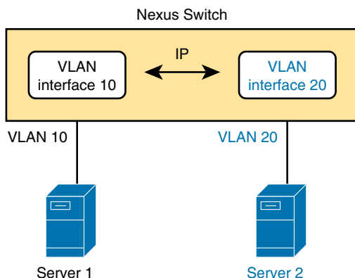
Figure 16-10 SVI Logically Represented on a Nexus Switch
