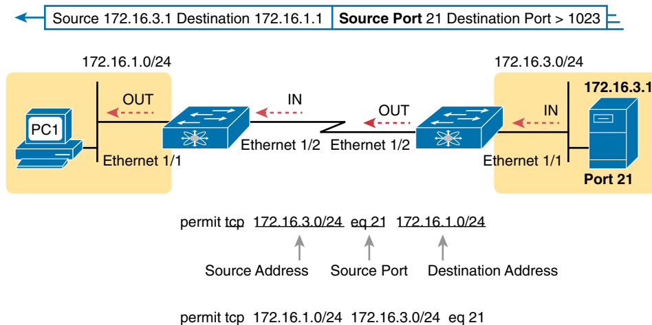
Figure 21-9 Filtering Packets Based on Source Port
