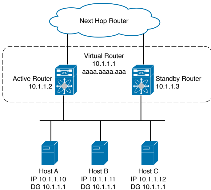
Figure 20-9 HSRP Topology
