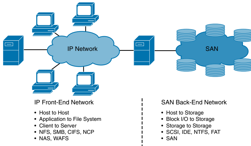
Figure 22-11 Block I/O Versus File I/O
