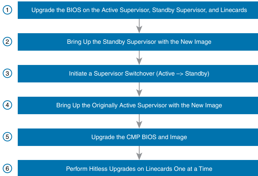
Figure 5-8 NX-OS ISSU Steps
