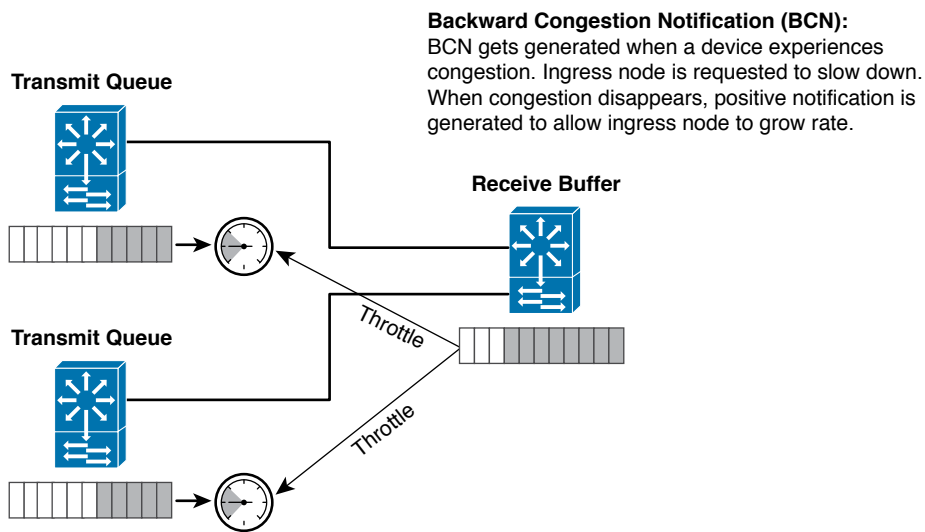
Figure 23-46 Congestion Notification
